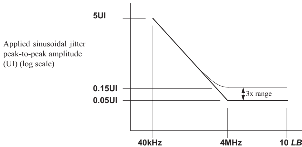
Figure 52–4—Mask of the sinusoidal component of jitter tolerance (informative)
